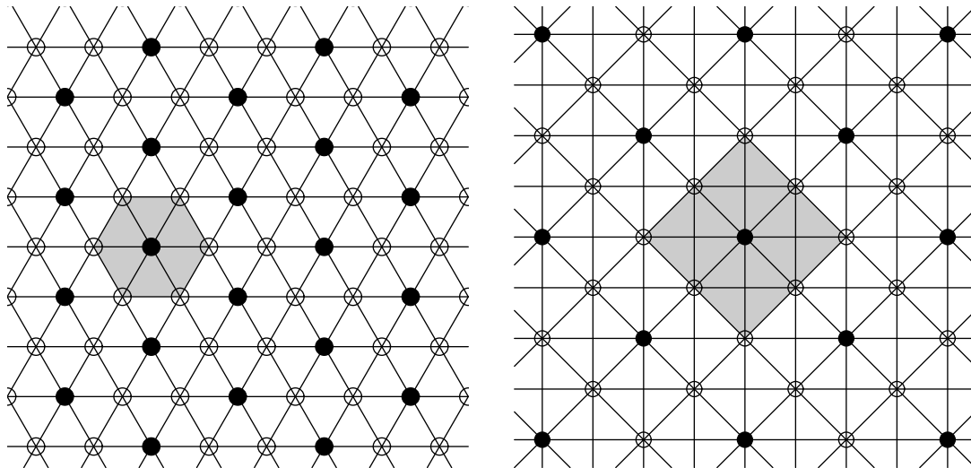
Figure 5. Left figure: The triangular lattice \mathcal{L} of units (indicated by small circles) for the kagomé lattice, showing an a -LM state with a = a_{\max} = \frac{1}{3}\ell_1 . The occupied units are indicated by filled circles. For this state the lattice \mathcal{L} can be filled by hexagons drawn around each occupied unit. One of these hexagons is shown in the figure. Right figure: The analogous figure for the checkerboard lattice. Here the lattice \mathcal{L} of units is a quadratic lattice with diagonals. The figure shows an a -LM state with a = a_{\max} = \frac{1}{4}\ell_1 . For this state the lattice \mathcal{L} can be filled by 4-squares drawn around each occupied unit. One of these 4-squares is shown in the figure.
