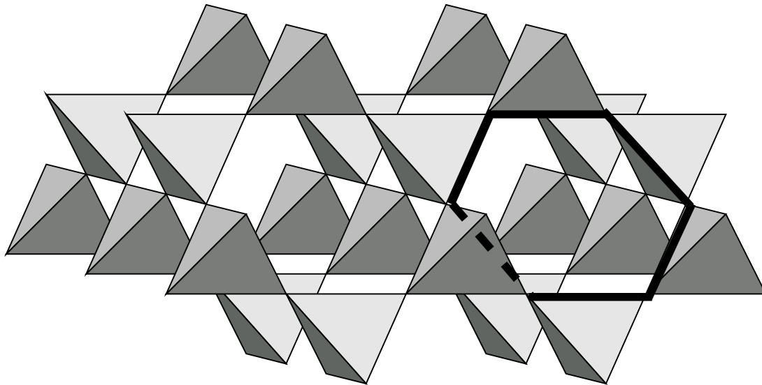
Figure 4. The pyrochlore lattice [20] as an example of a spin lattice admitting a -LM states satisfying more than one linear relation (higher codimension type). All exchange constants are positive and equal. 1-LM states are localized on small hexagonal subsystems (“units”) typically indicated by thick lines.
