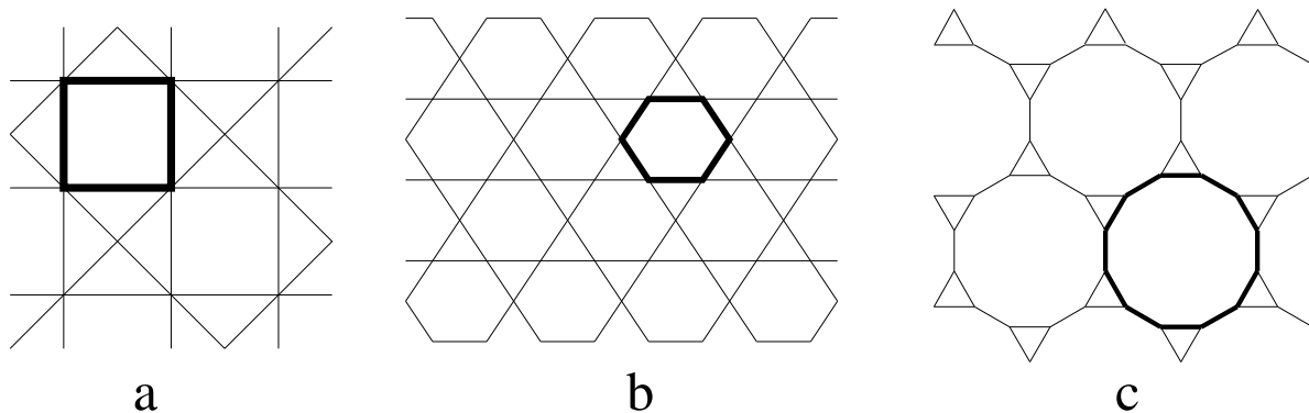
Figure 3. Examples of spin lattices admitting only 1-LM states satisfying exactly one linear relation (codimension one type): (a) the checkerboard lattice or two-dimensional pyrochlore [17] (where the spins are sitting only on the squares, not on the intersections of the diagonals), (b) the kagomé lattice [18, 3], and (c) the star lattice [3, 19]. All exchange constants are positive and equal. 1-LM states are localized on small subsystems (“units”) typically indicated by thick lines.
