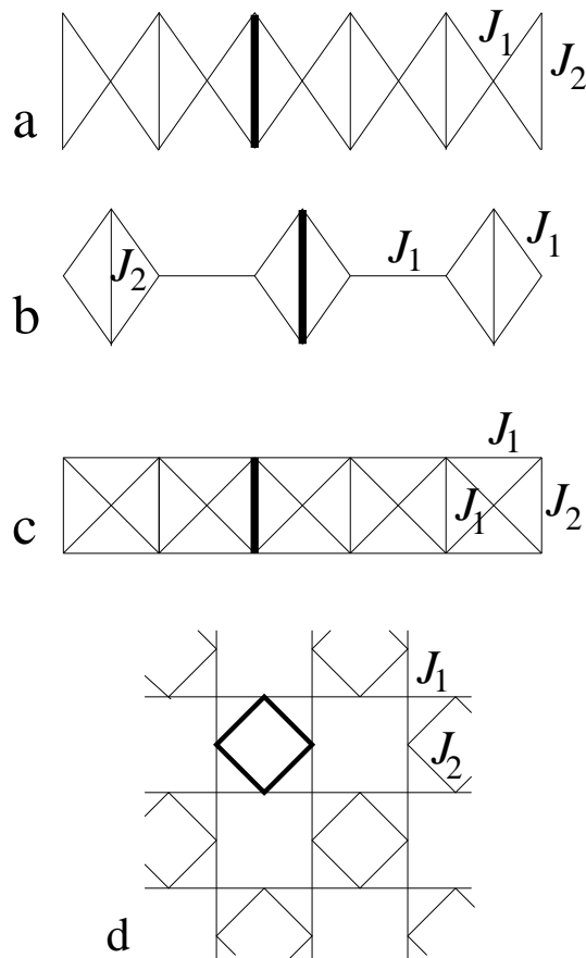
Figure 1. Examples of spin lattices admitting only orthogonal LM states (orthogonal type): (a) the diamond chain [10], (b) the dimer-plaquette chain [11], (c) the frustrated ladder [12] (where the spins are sitting only on the squares, not on the intersections of the diagonals) and (d) the square-kagomé lattice [13]. Note that the ratios of the exchange constants J_1, J_2 have to assume certain values in order to admit LM states, for more details see Ref. [8]. 1-LM states are localized on small subsystems (“units”) typically indicated by thick lines.
