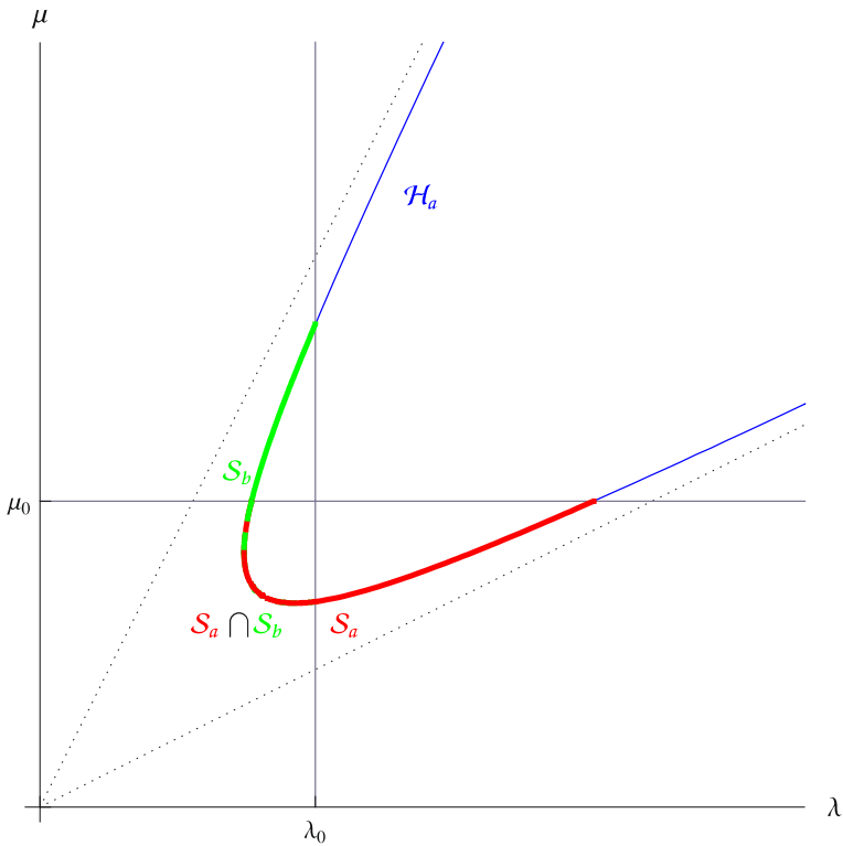
Fig. 3 One branch \mathcal{H}_a of the hyperbola described by Eq. 75 together with the segments \mathcal{S}_a and \mathcal{S}_b defined by \mu \leq \mu_0 and \lambda \leq \lambda_0 , respectively. To every point in \mathcal{S}_a \cap \mathcal{S}_b there exist effects a and b satisfying Eq. 1 and hence e and f are coexistent
