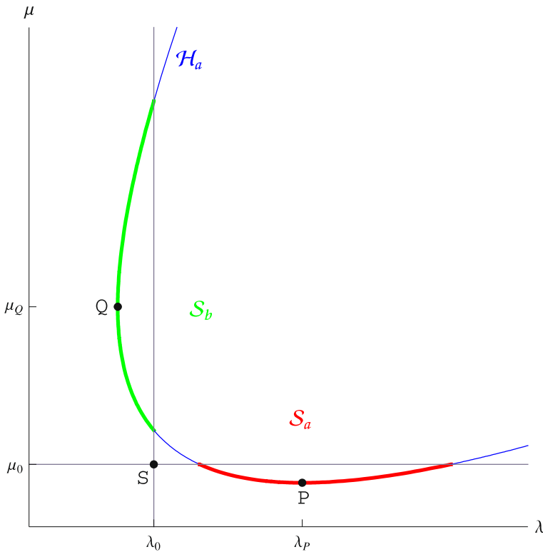
Fig. 4 The only case where S_a \cap S_b = \emptyset occurs if and only if \lambda_0 < \lambda_P and \mu_0 < \mu_Q and S = (\lambda_0, \mu_0) lies outside the convex hull of the hyperbola branch \mathcal{H}_a
