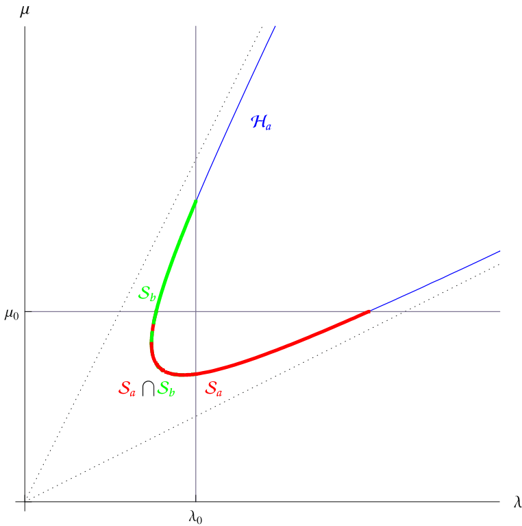
Fig. 3 One branch \mathcal{H}_a of the hyperbola described by Eq. 75 together with the segments S_a and S_b defined by \mu \leq \mu_0 and \lambda \leq \lambda_0 , respectively. To every point in S_a \cap S_b there exist effects a and b satisfying Eq. 1 and hence e and f are coexistent
