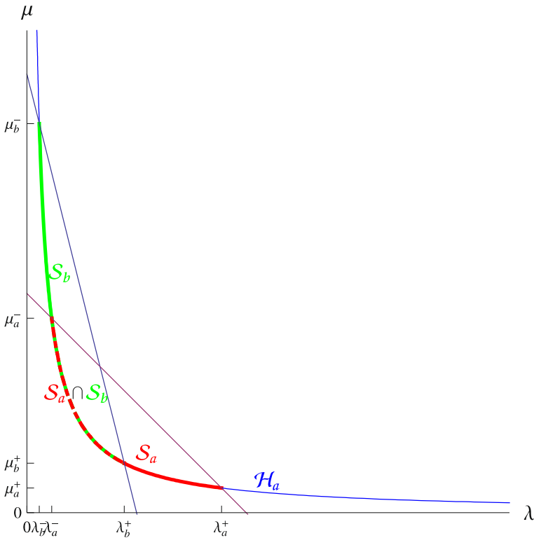
Fig. 2 Representation of the hyperbola branch \mathcal{B}(e) \cap \mathcal{B}(f) in the \lambda - \mu -plane, with an indication of the coordinates of the end points of the segments \mathcal{S}_a, \mathcal{S}_b
